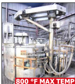
800 °F MAX TEMP SURFACE pit draw furnace
