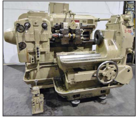
FARREL 2C gear cutter
