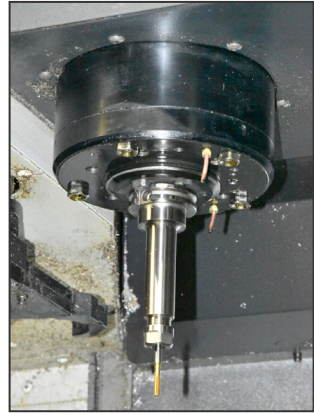
View of MORI SEIKI spindle
