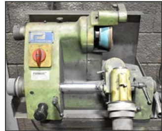
PREGRAPH tool and cutter grinder
