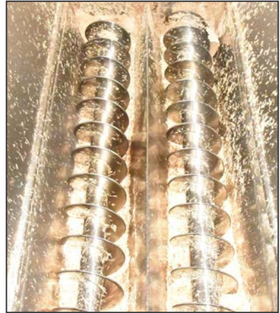
View of chip bin twin auger feed screws
