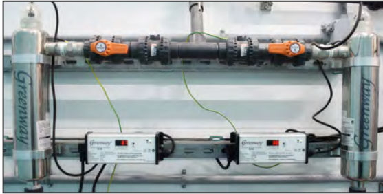
GREENWAY GUVL-330S electronic germicidal UV sterilization system
