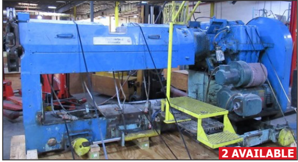
DAVIS STANDARD 35IN35 3.5" capacity single screw plastic extruder
