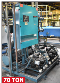
70 TON BERG ASR-70-1/2 skid mounted industrial chiller
