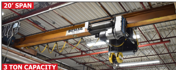
20' SPAN 3 TON CAPACITY DEMAG single girder top-running overhead bridge crane
