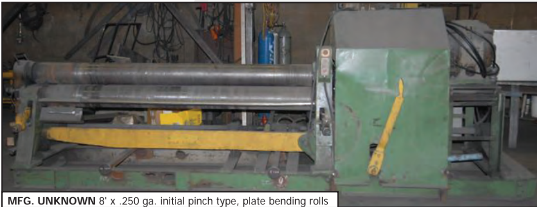
MFG. UNKNOWN 8' x .250 ga. initial pinch type, plate bending rolls
