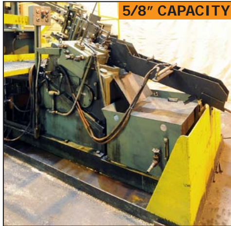
SAKAMURA SSR 50 planetary thread roller
