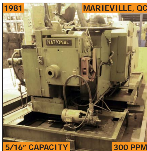
NATIONAL 5S3 high speed 3 die bolt maker
