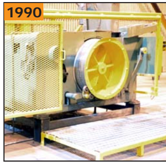
5/8" RMG 910-4081-2 wire drawer
