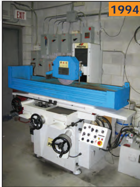
PROTH PSGS-3060AH automatic hydraulic surface grinder with 12"x24" chuck s/n 40807-15
