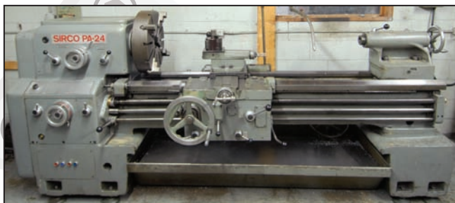
SIRCO PA-24 gap bed engine lathe
