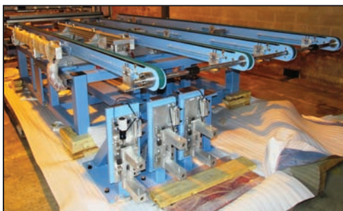
QASR 18 GRENZBACH infeed conveyor unit
