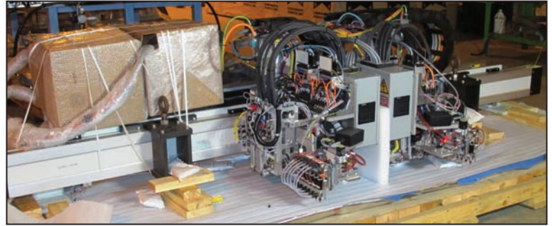
BUSLINE cross bus gantry
