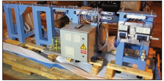
BUSLINE gantry mounting bkts, 4XEFD valve-matic 8000 fluid dispensing unit w/FESTO pneumatic valve bank
