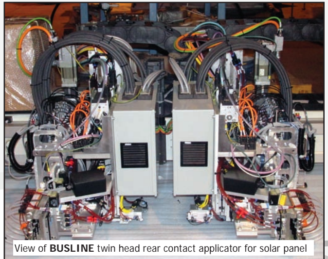
View of BUSLINE twin head rear contact applicator for solar panel
