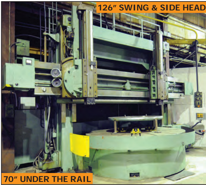
STANKO IL532 vertical boring mill
