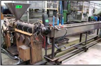
TTS automatic wire coating line
