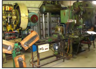
TTS automatic TAC strip manufacturing line
