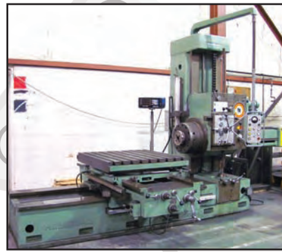
MEUSER 3" table type horizontal boring mill
