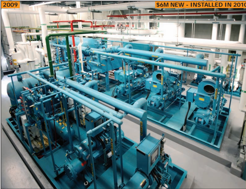
Partial view of TORONTO CIMCO 455TR & 42TR AMMONIA/GLYCOL REFRIDGERANT SYSTEMS
